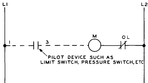
2 WIRE CONTROL
