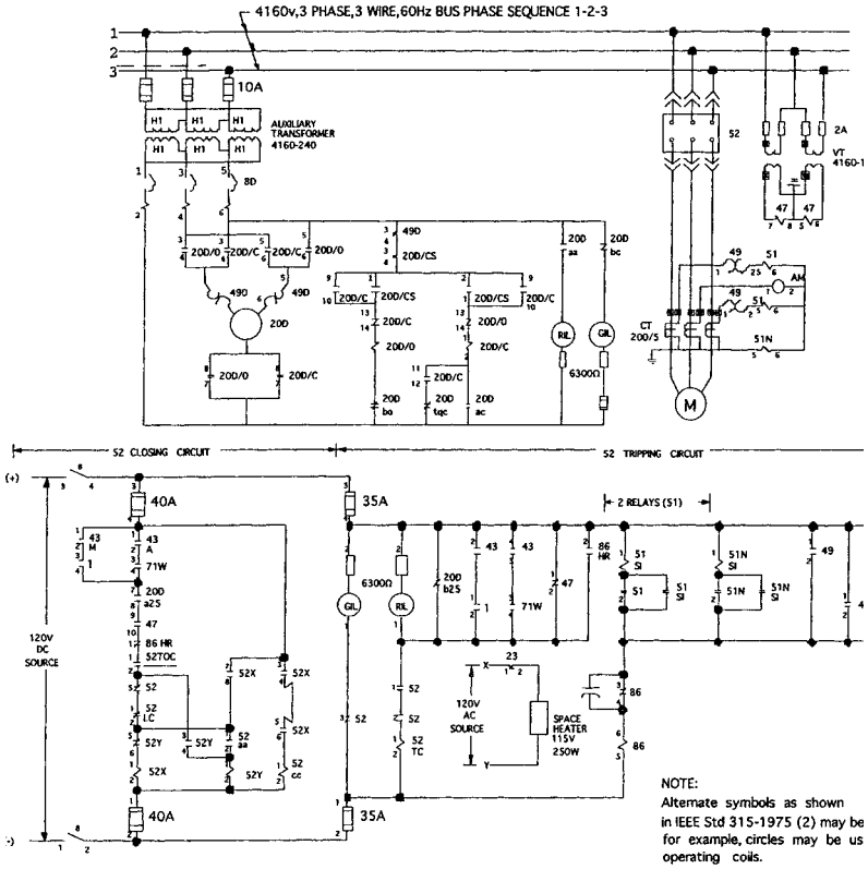
Figure 4— Typical elementary diagram
