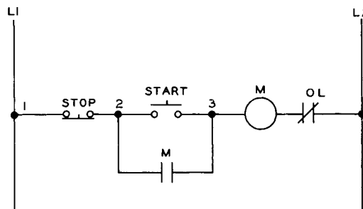
3 WIRE CONTROL
