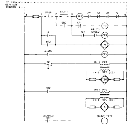
Solid State Reduced Voltage Controllers with a Shorting Contactor and an Isolation Contactor MJ(320A), MK(500A) and MM(750A) Devices
