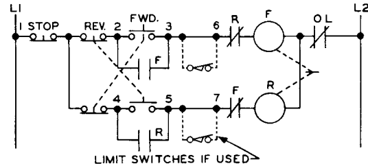
3 WIRE CONTROL - REVERSING STARTER
