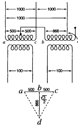
Two single-phase transformers connected T to a three-phase two-phase system. Scott Connection.
