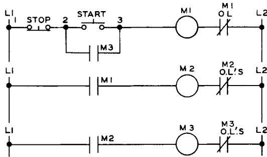
3 WIRE CONTROL - MORE THAN ONE STARTER, ONE PUSH BUTTON STATION CONTROLS ALL
