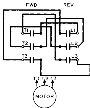
Type K, 3 Pole, 3 Phase
