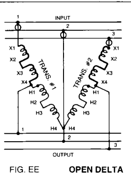
FIG. EE OPEN DELTA
