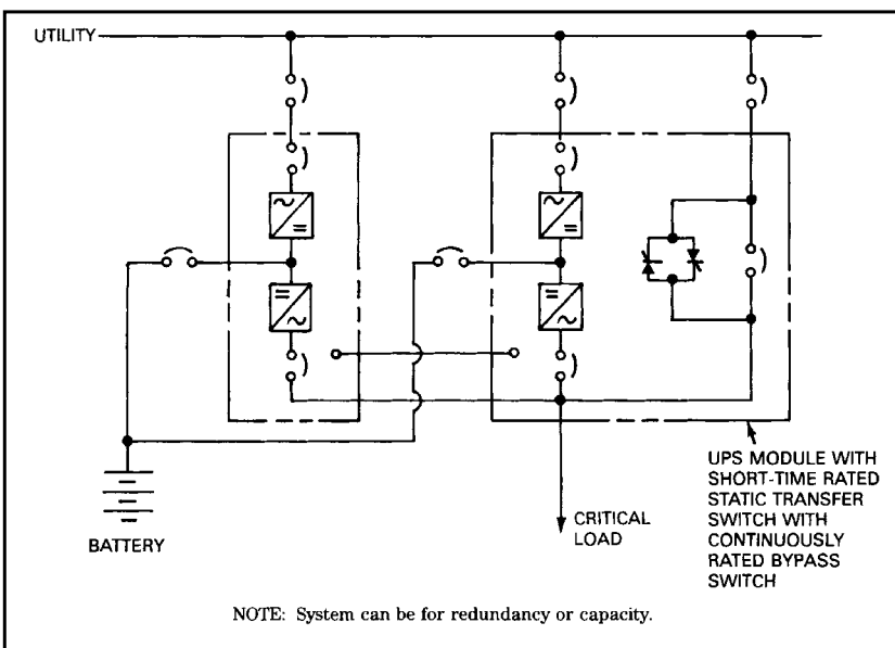
FIGURE 5.19 Parallel tandem UPS system. (From IEEE Std. 241-1990. Copyright 1990 IEEE. All rights reserved.)
