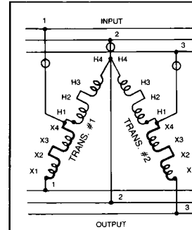
FIG. BB OPEN DELTA
