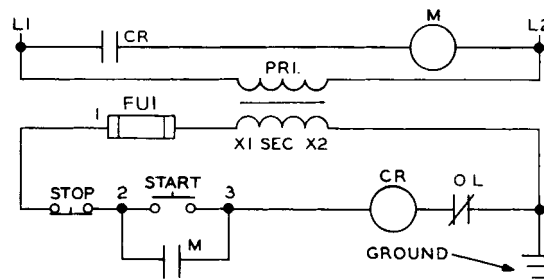
3 WIRE CONTROL WITH FUSED CONTROL CIRCUIT TRANSFORMER AND CONTROL RELAY
